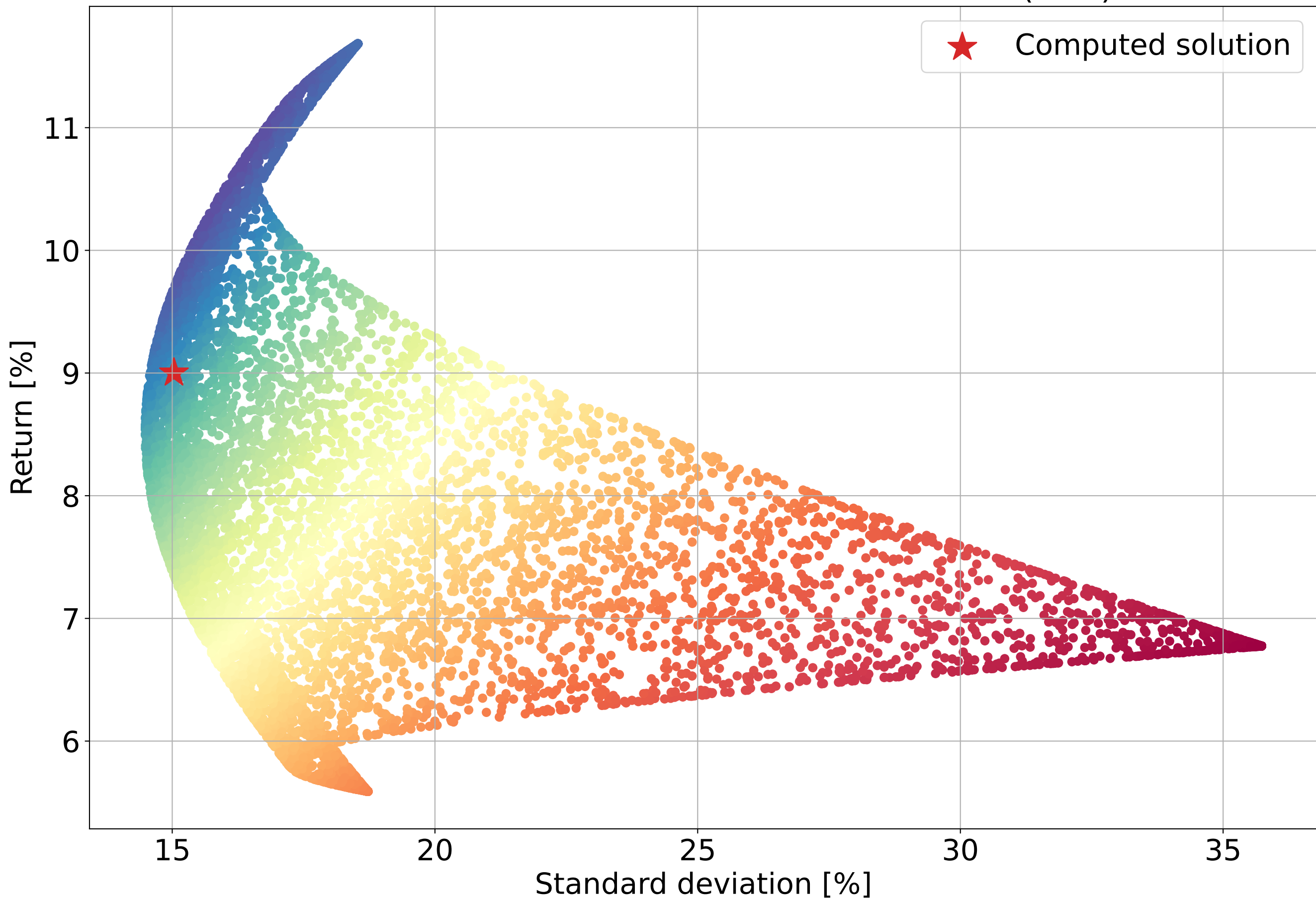
Montecarlo on Ytest -- Markovitz Probabilistic (n=3)
